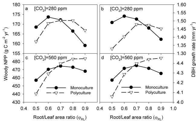
Figure 10. Woody NPP and DBH growth rates in monoculture and polyculture models runs at (a–b) [CO 2 ] = 280 ppm, and (c–d) [CO 2 ] = 560 ppm. PFTs differed only their allocation to fine roots ( \varphi_{RL} ; see Fig. 8 legend for explanation). The optimal monoculture is defined as the type with the highest woody NPP (which, given the allometries in LM3-PPA, is also the type with the highest DBH growth rate) when grown in monoculture. In this figure, the competitive optimum is identified as the type with the highest woody NPP (or highest DBH growth rate) in polyculture model runs. Figures 8–10 present multiple ways to identify the competitive optimum (i.e., the convergence-stable ESS), and all yield consistent results: \varphi_{RL} = 0.7 and \varphi_{RL} = 0.9 at 280 and 560 ppm, respectively.
